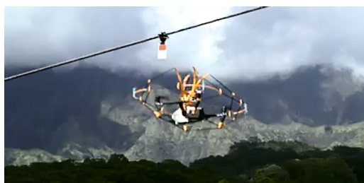
FireFly diverters can be installed by drone
