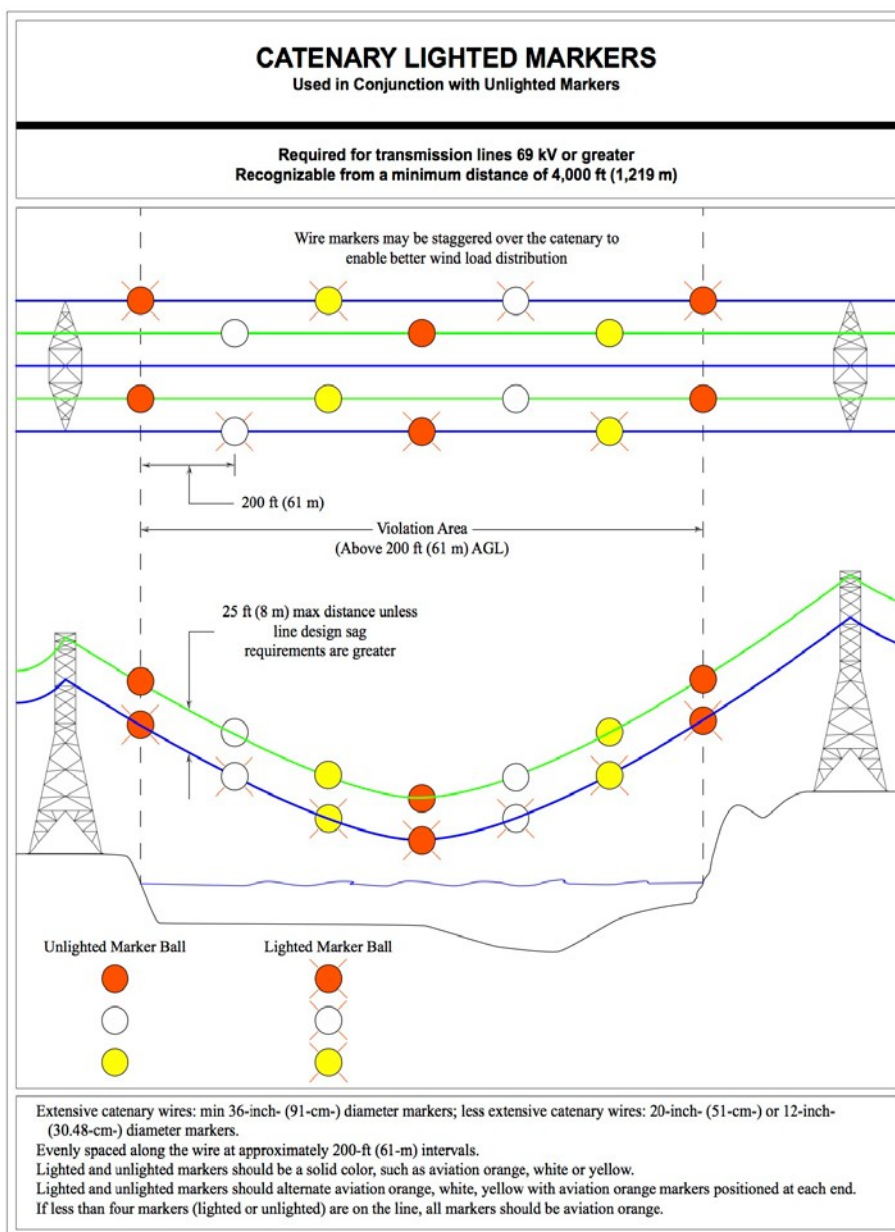
Figure A-24. Catenary Lighted Markers
