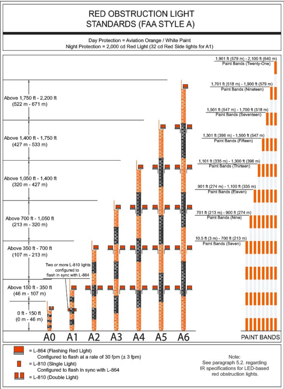
Figure A-6. Red Obstruction Light Standards
