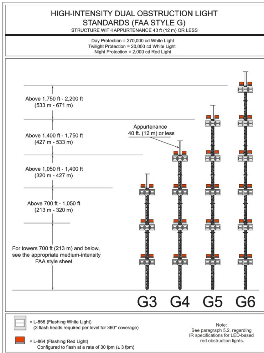
Figure A-19. High-Intensity Dual Obstruction Lighting Standards—Structures With Appurtenance 40 Feet or Less
