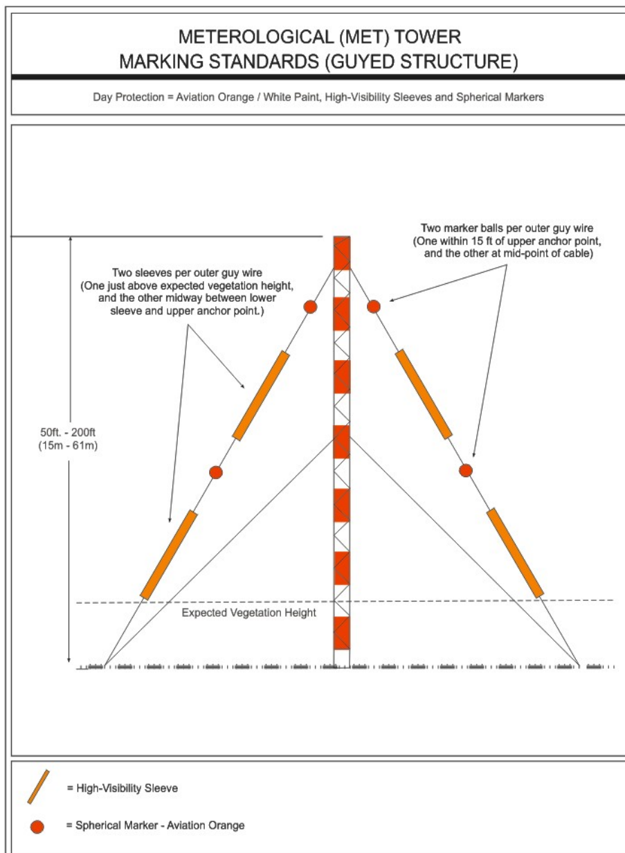
Figure A-2. Meteorological (MET) Tower Marking Standards (Guyed Structure)
