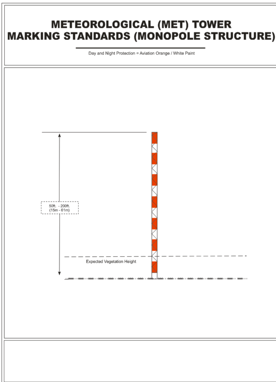
Figure A-1. Meteorological (MET) Tower Marking Standards (Monopole Structure)
