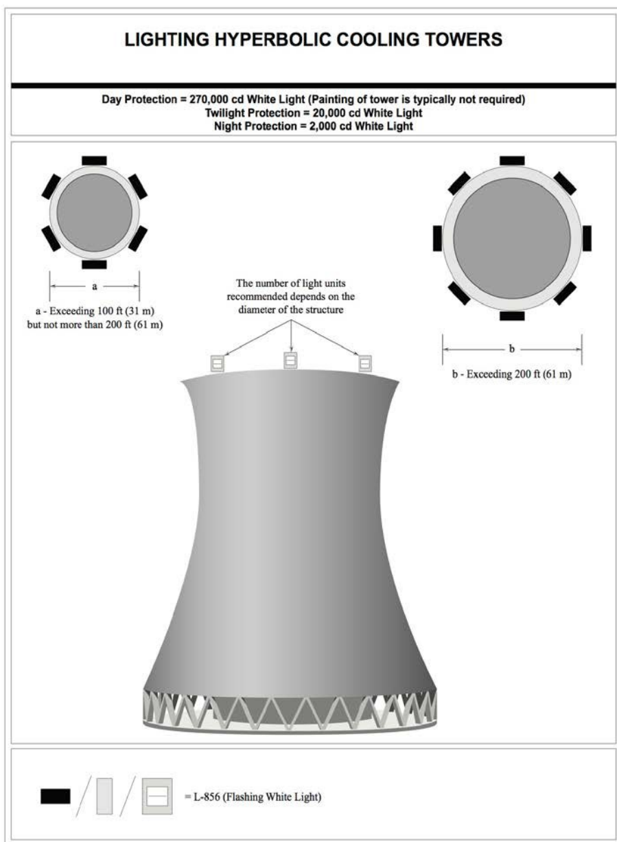
Figure A-15. Hyperbolic Cooling Tower
