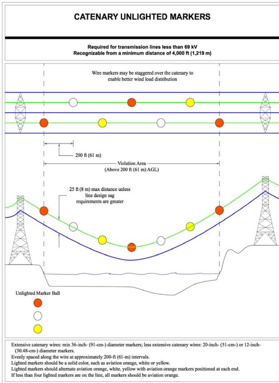
Figure A-21. Catenary Unlighted Markers
