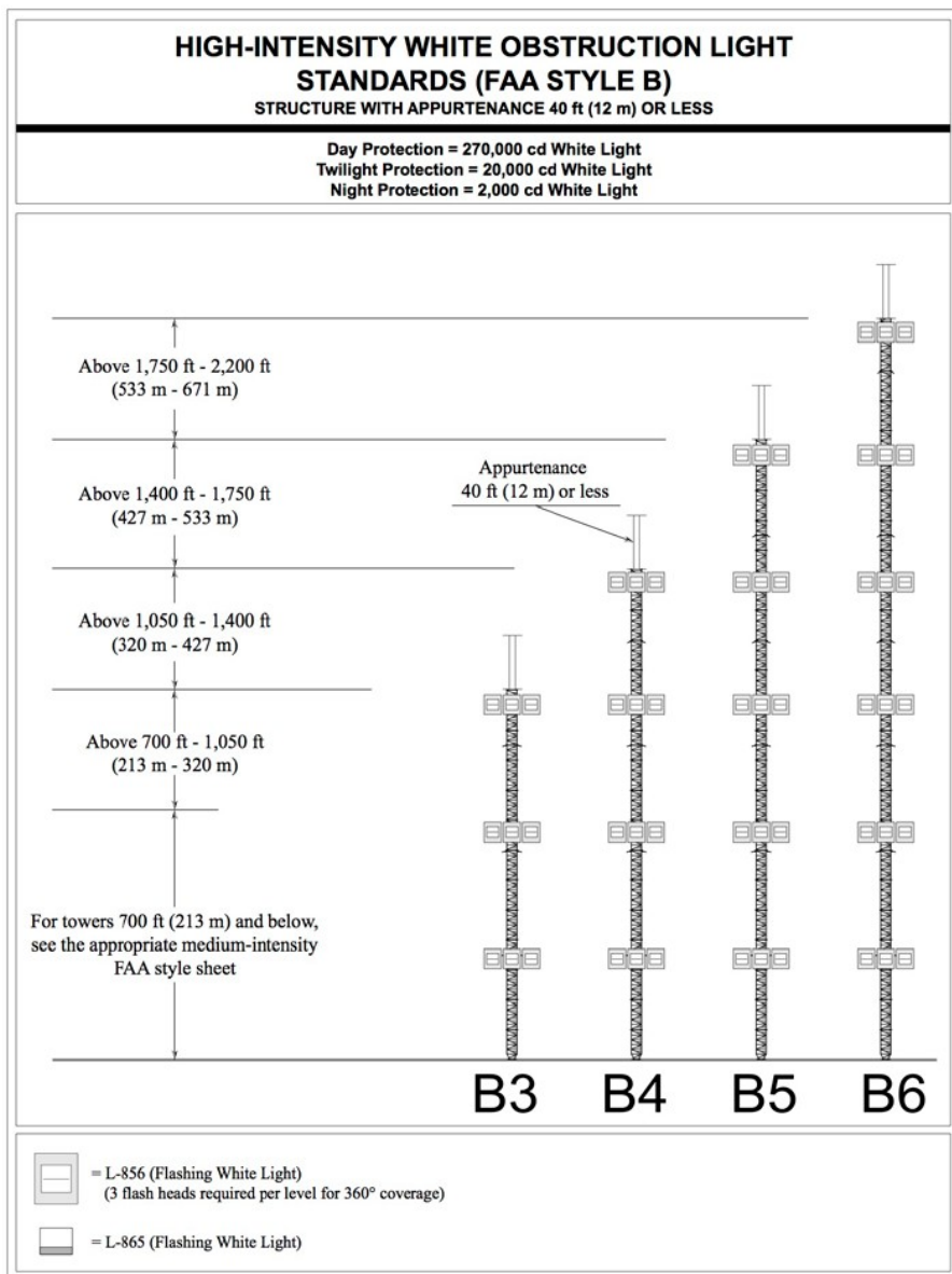
Figure A-13. High-Intensity White Obstruction Light Standards—Structures With Appurtenance 40 Feet or Less
