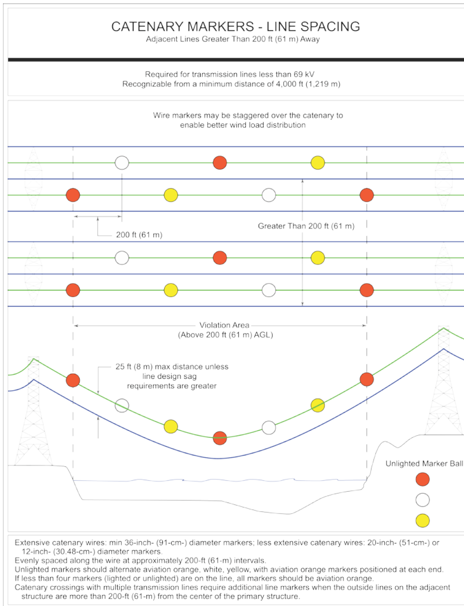
Figure A-23. Catenary Markers - Line Spacing (Adjacent Lines Greater Than 200 ft. (60.96 m) Away)
