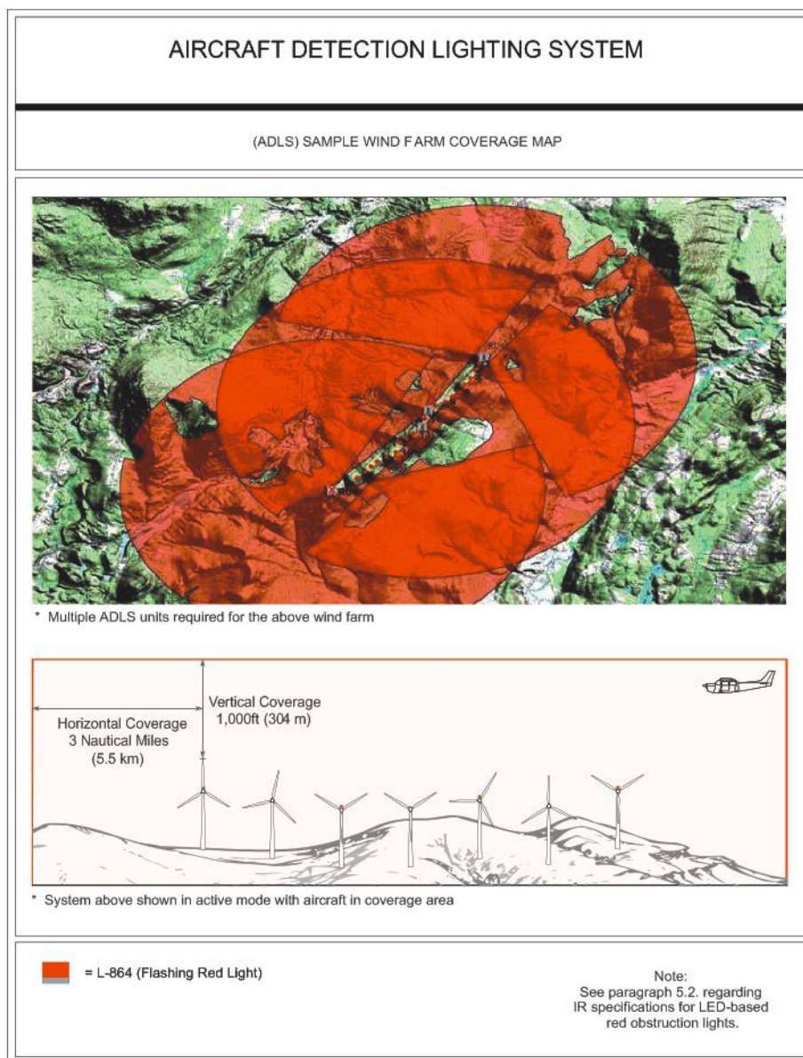
Figure A-20. Sample of Aircraft Detection Lighting System Coverage Map
