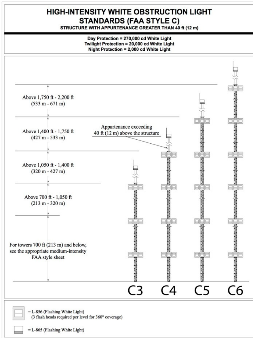
Figure A-14. High-Intensity Obstruction Lighting Standards—Structures With Appurtenance Over 40 Feet High
