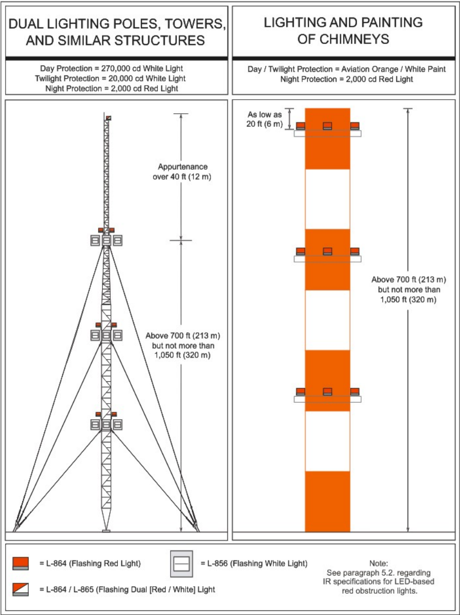
Figure A-7. Painting and/or Dual Lighting of Chimneys, Poles, Towers, and Similar Structures
