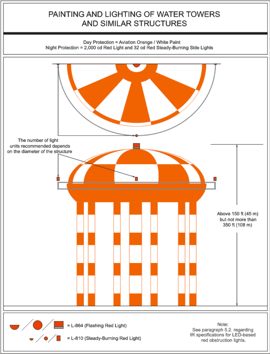
Figure A-4. Painting and Lighting of Water Towers and Similar Structures
