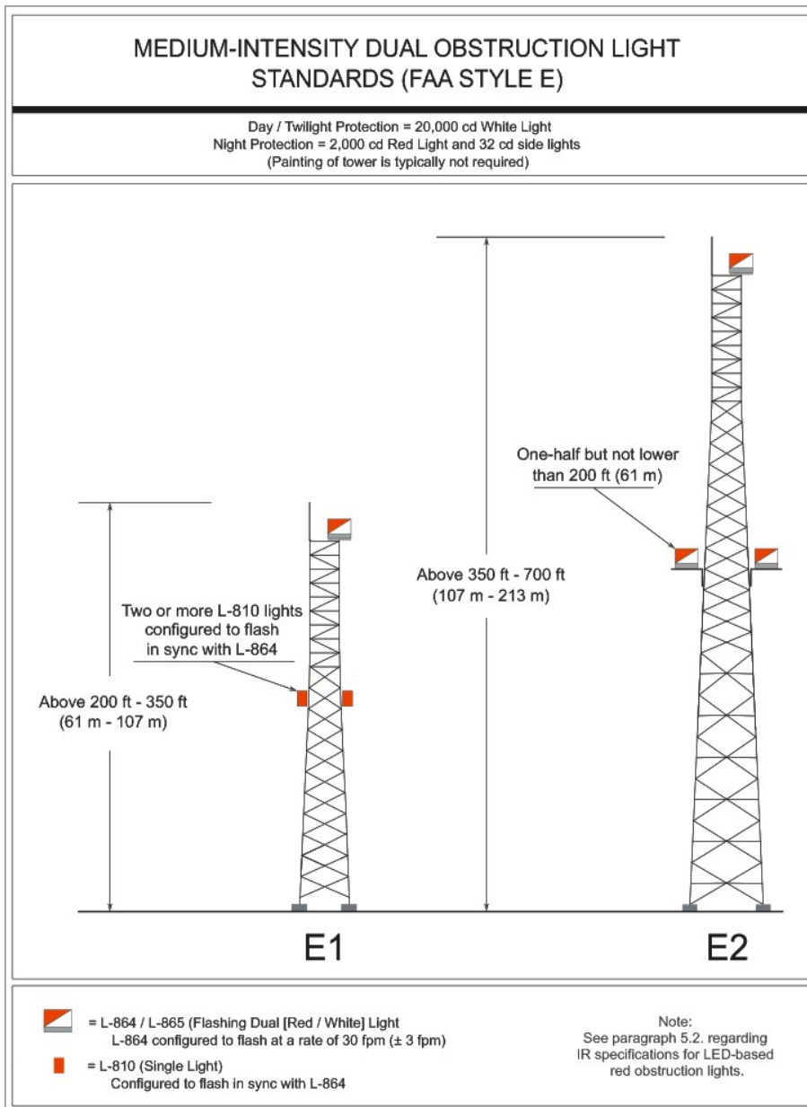
Figure A-16. Medium-Intensity Dual Obstruction Lighting Standards
