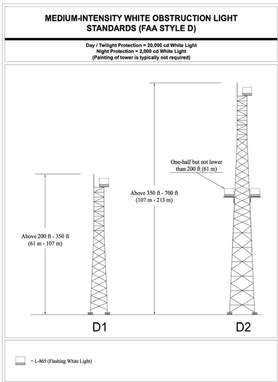
Figure A-9. Medium-Intensity White Obstruction Light Standards
