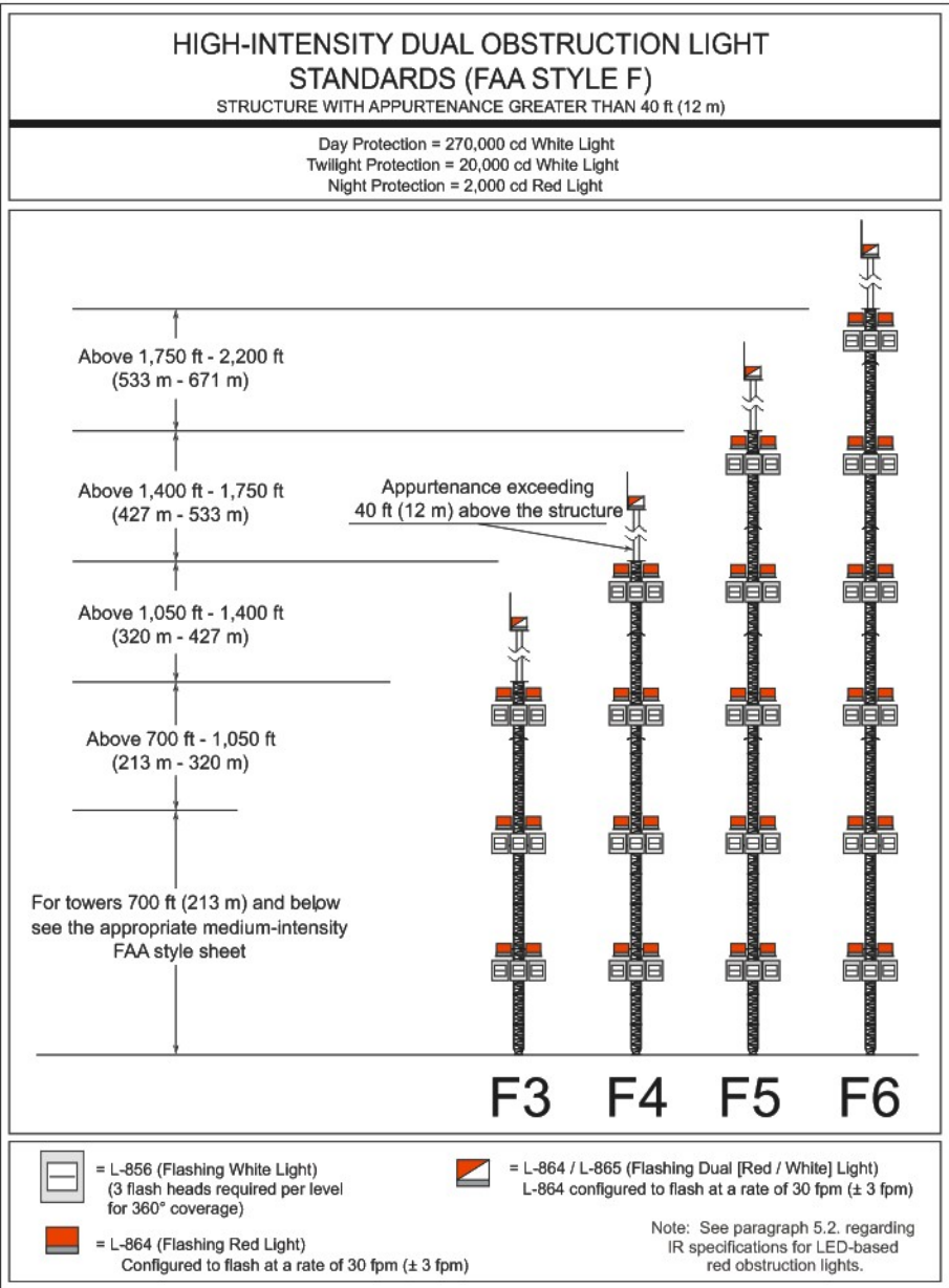
Figure A-18. High-Intensity Dual Obstruction Lighting Standards—Structures With Appurtenance Over 40 Feet High
