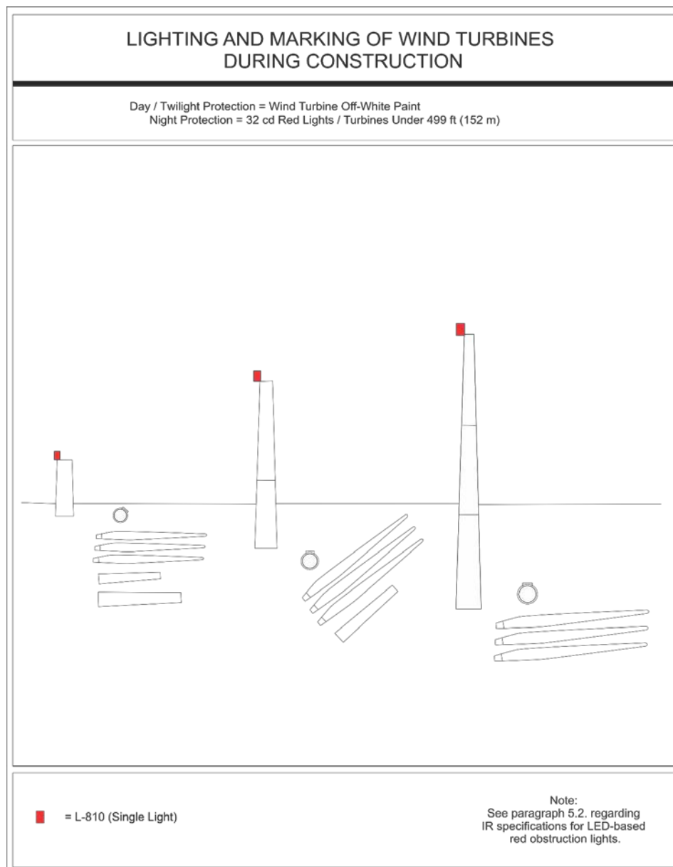
Figure A-30. Sample of Marking and Lighting for Turbine During Construction
